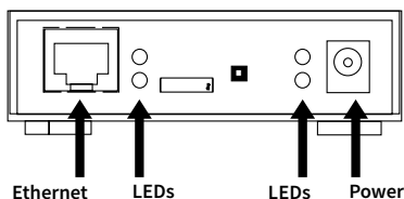
PORTSERVER TS MEI FAMILY - FRONT
